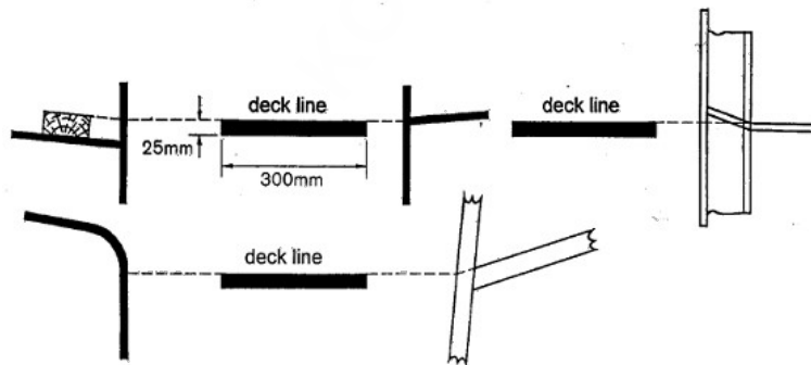
Figure 4.1 Deck line
